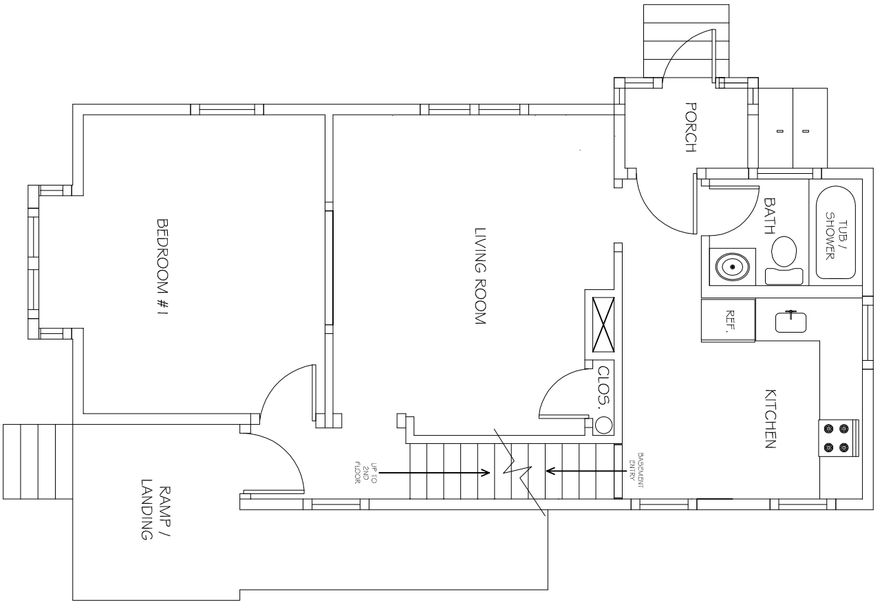
1ST FLOOR PLAN 109 CROSS STREET
